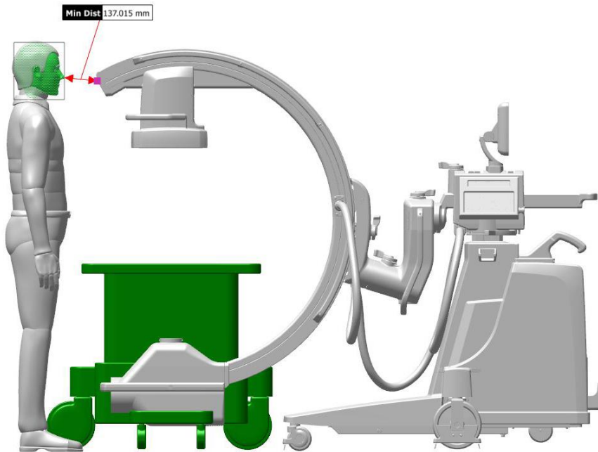
Figure 3. Theoretical position of surgeon while operating on a patient if steel counterweights are used. This is impossible as the edge of the C-arm prevents the surgeon from standing over the patient and so they would not be able to view them properly
