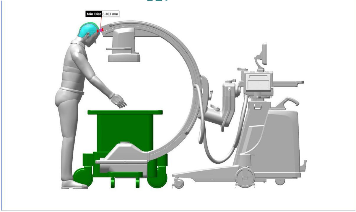
Figure 1. Position of surgeon when operating on a patient. There is a 6.4mm gap between their head and the edge of the c-arm when lead counterweights are used
